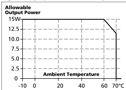
Fig. 16-1 Output power vs. ambient temperature
