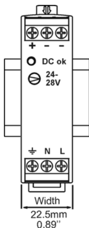
Fig. 23-1 Front view
