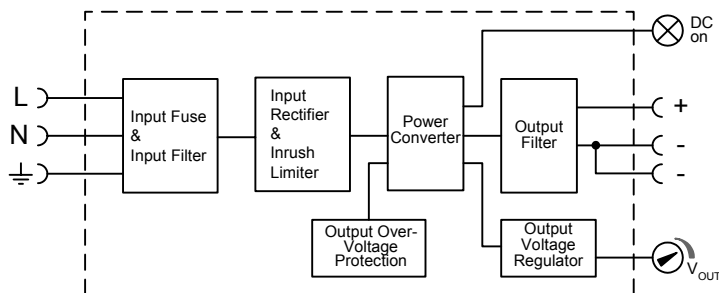
Fig. 11-1 Functional diagram
