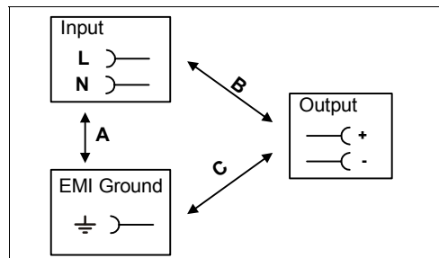
Fig. 19-1 Dielectric strength
