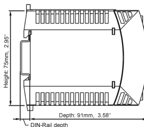
Fig. 23-2 Side view
