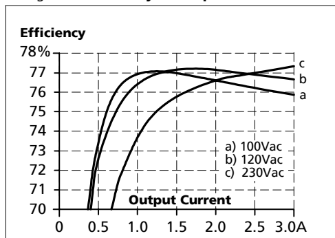
Fig. 10-1 Efficiency vs. output current at 5V
