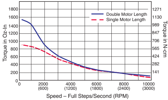
MDrive42AC – 120VAC
