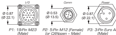
Connectors
