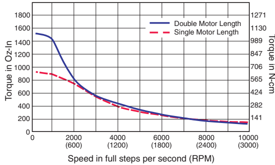
MDrive42AC – 240VAC
